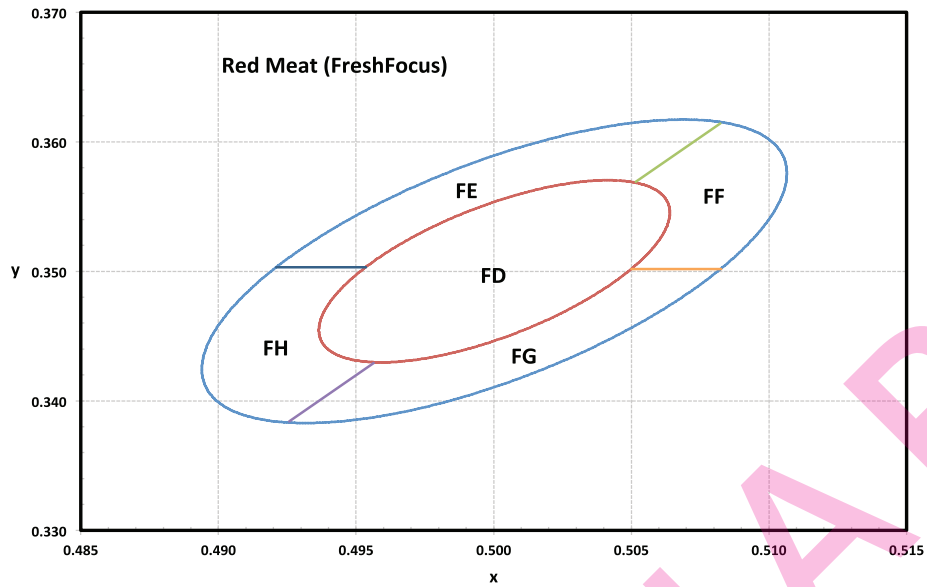
Figure 8b. 1/5 th color bin structure for LUXEON 2835C with FreshFocus Technology for Red Meat, 120mA, T_j=25^\circ\text{C} .
