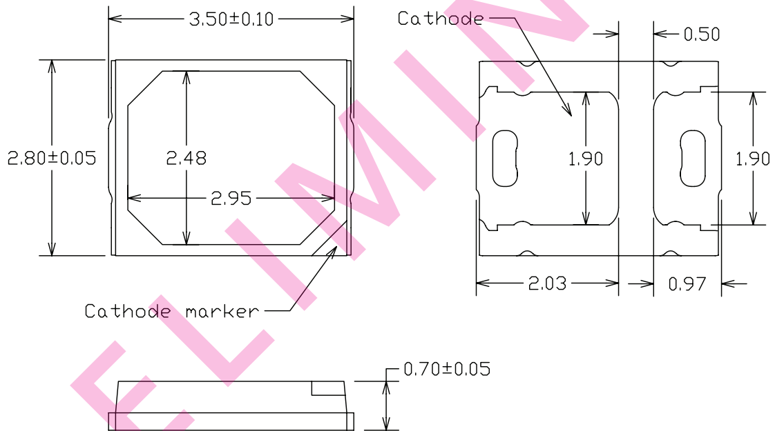
Figure 9. Mechanical dimensions for LUXEON 2835C with FreshFocus Technology.
