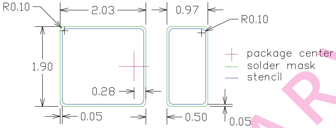
Figure 11. Recommended PCB solder pad layout for LUXEON 2835C with FreshFocus Technology.
