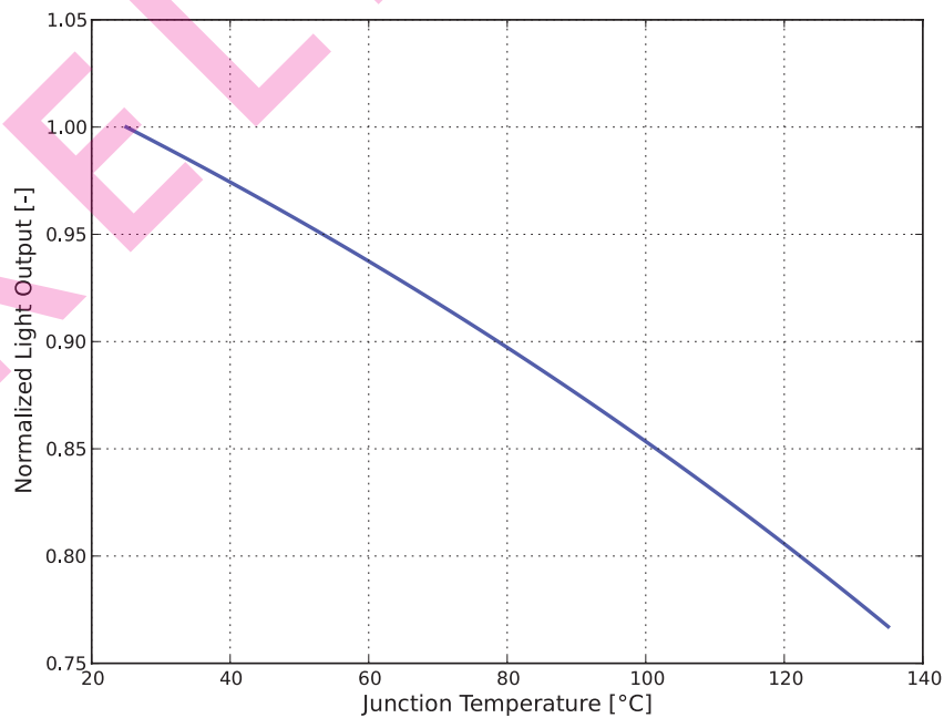
Figure 2. Typical normalized light output vs. junction temperature for LUXEON 2835C with FreshFocus Technology at 120mA.
